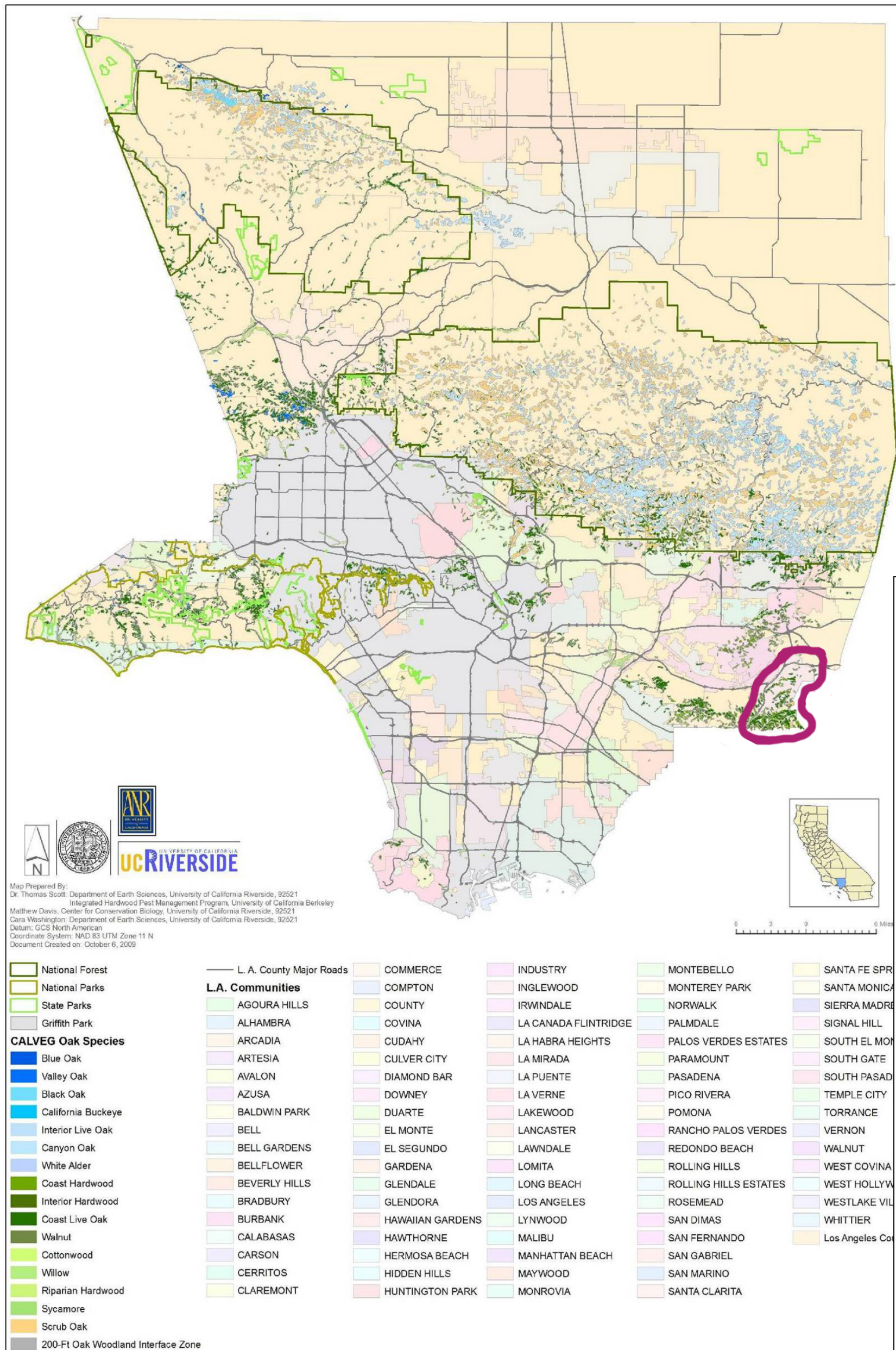
FIGURE A2 – DISTRIBUTION OF OAK SPECIES IN LOS ANGELES COUNTY
